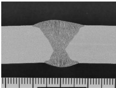
DW-308L-XR 0.045" 200A-29V 75%Ar-25%CO 2
